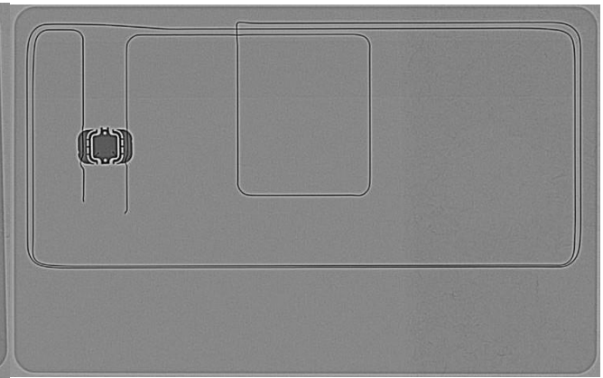
CPI card for ISO14443 Type B
