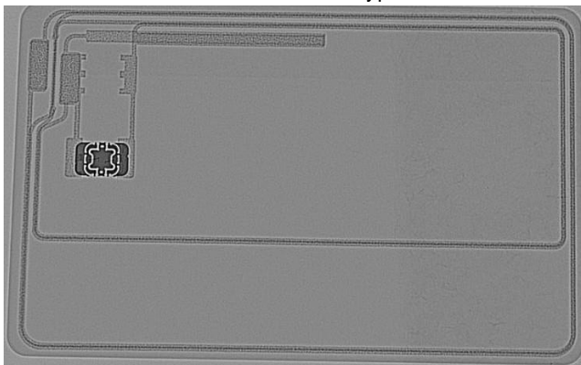
G & D card for ISO14443 Type A
