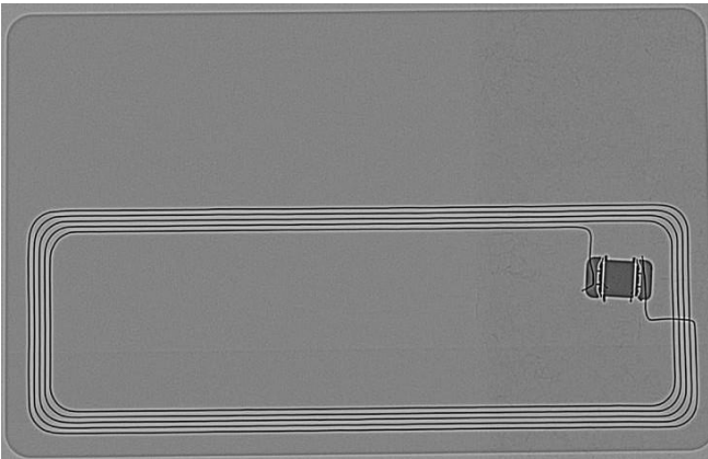
GemPlus (Gemalto) card for ISO14443 Type B
